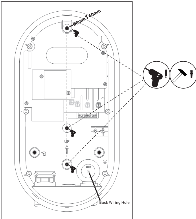
Figure 2-4 Locate the installation location for pole-mounted
