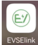
Figure 3-1 EVSElink app
